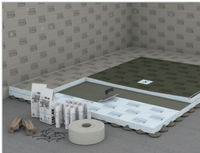
e.g. MODUL-ROOM 1800 KIT 1
