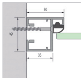
frame profile, wall connection
