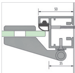
frame profile door hinge, wall connection
