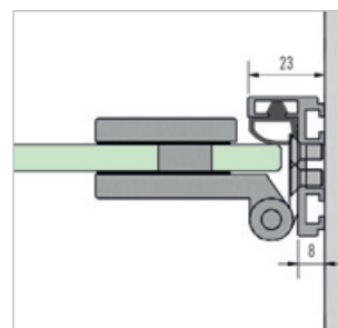
frame profile door hinge, wall connection
