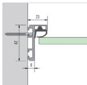
frame profile, wall connection
